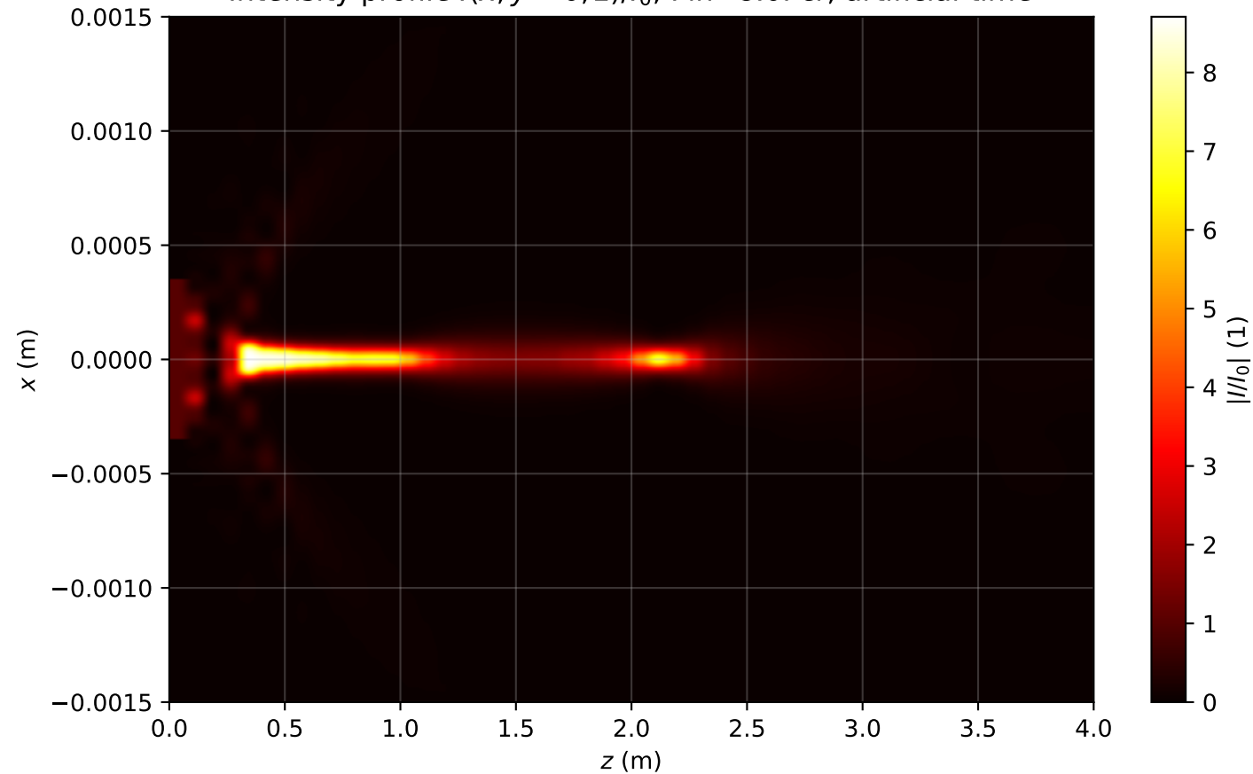
Intensity profile I(x, y = 0, z)/I_0 , P_{in}=8.0P_{cr} , artificial time
